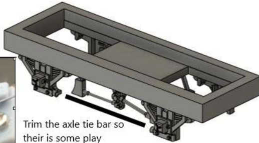
Axle assembly
